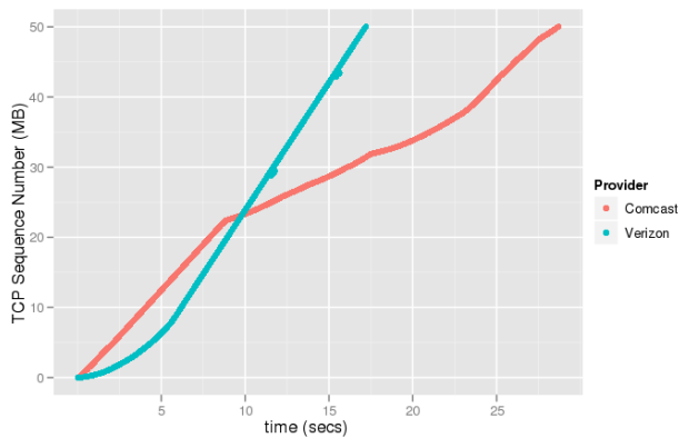
Figure 1: TCP sequence number plot comparing the download of a 50MB file on a Comcast 12 Mbps tier with Powerboost to a Verizon 25 Mbps FiOS tier. An artificial delay of 10 ms was added to the Comcast line using Linux netem so that both connections faced a ~20ms RTT to the server hosting the file.
